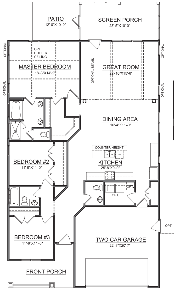
First Floor
