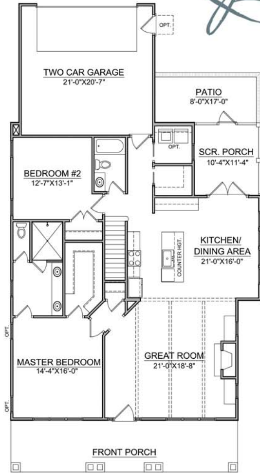
FLOOR PLAN
