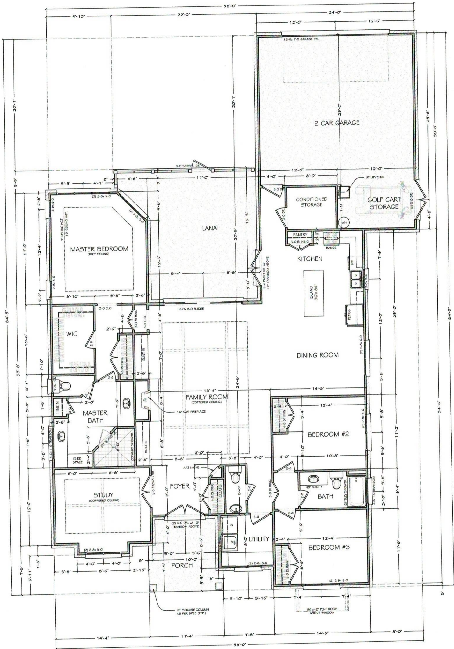
FLOOR PLAN SCALE: 1/4" = 1'-0"
